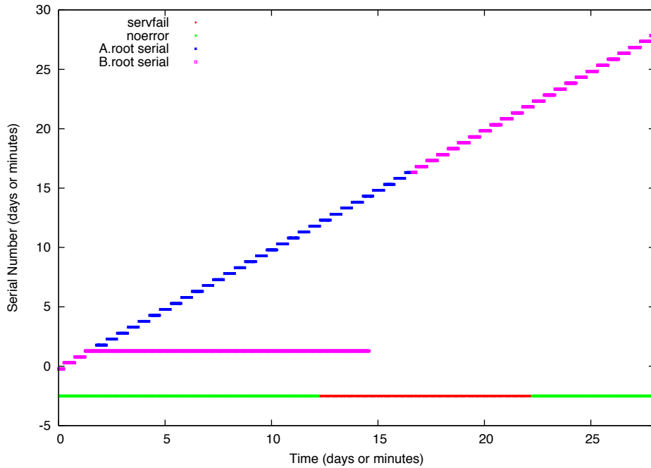
Figure 10: Simulation results demonstrating the ZSK signature validity problem. Green points represent successful queries, while red points represent SERVFAIL responses. Blue and purple points represent SOA serial values from the A and B root servers.
